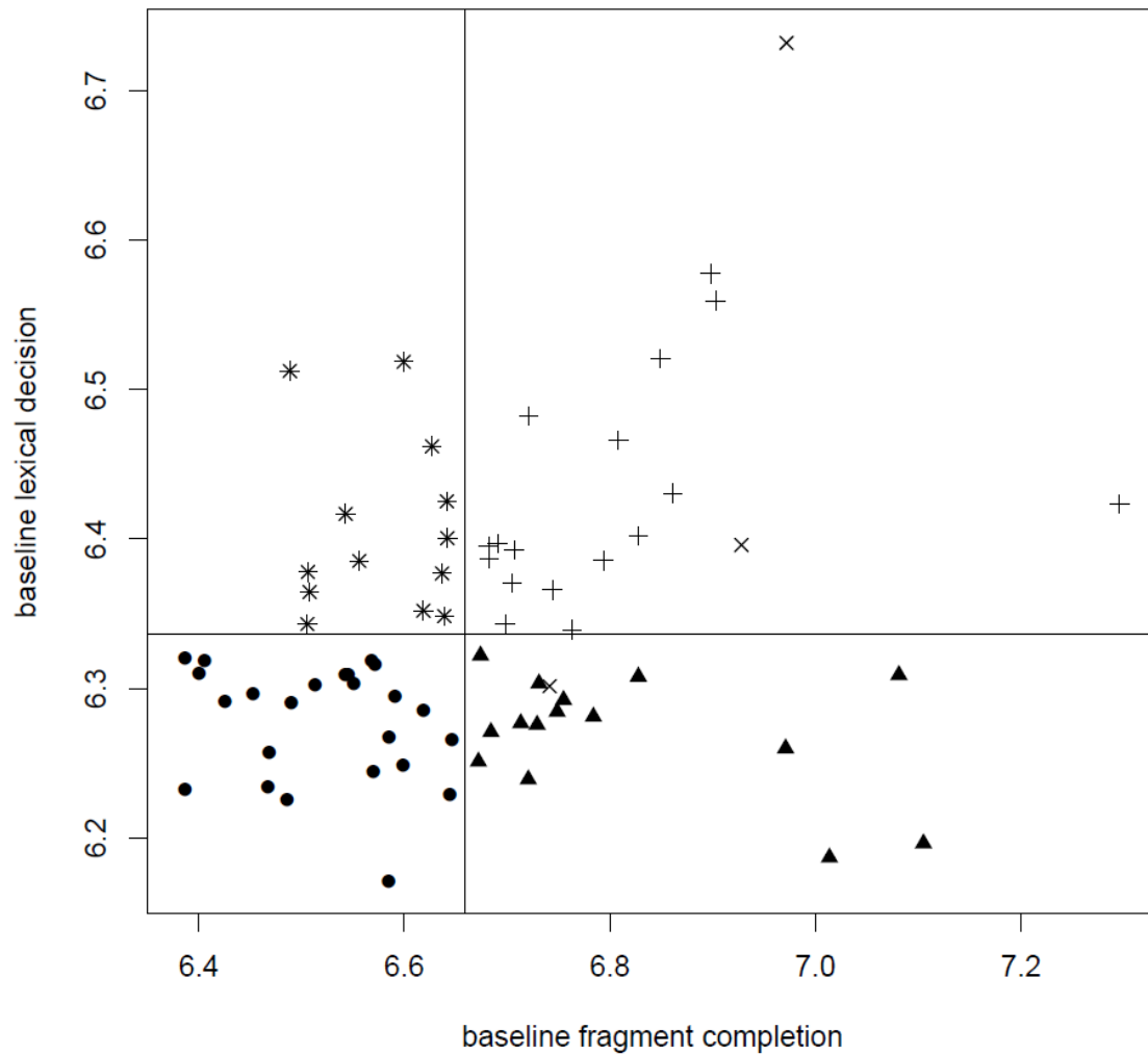
Figure 5. Average log-transformed response time in the unrelated condition for every item in the speeded word fragment completion task and the lexical decision task. Every symbol represents an item. The black lines indicate the grand average for each respective task, thereby creating quadrants. Items get a different symbol depending on their position in those quadrants.
