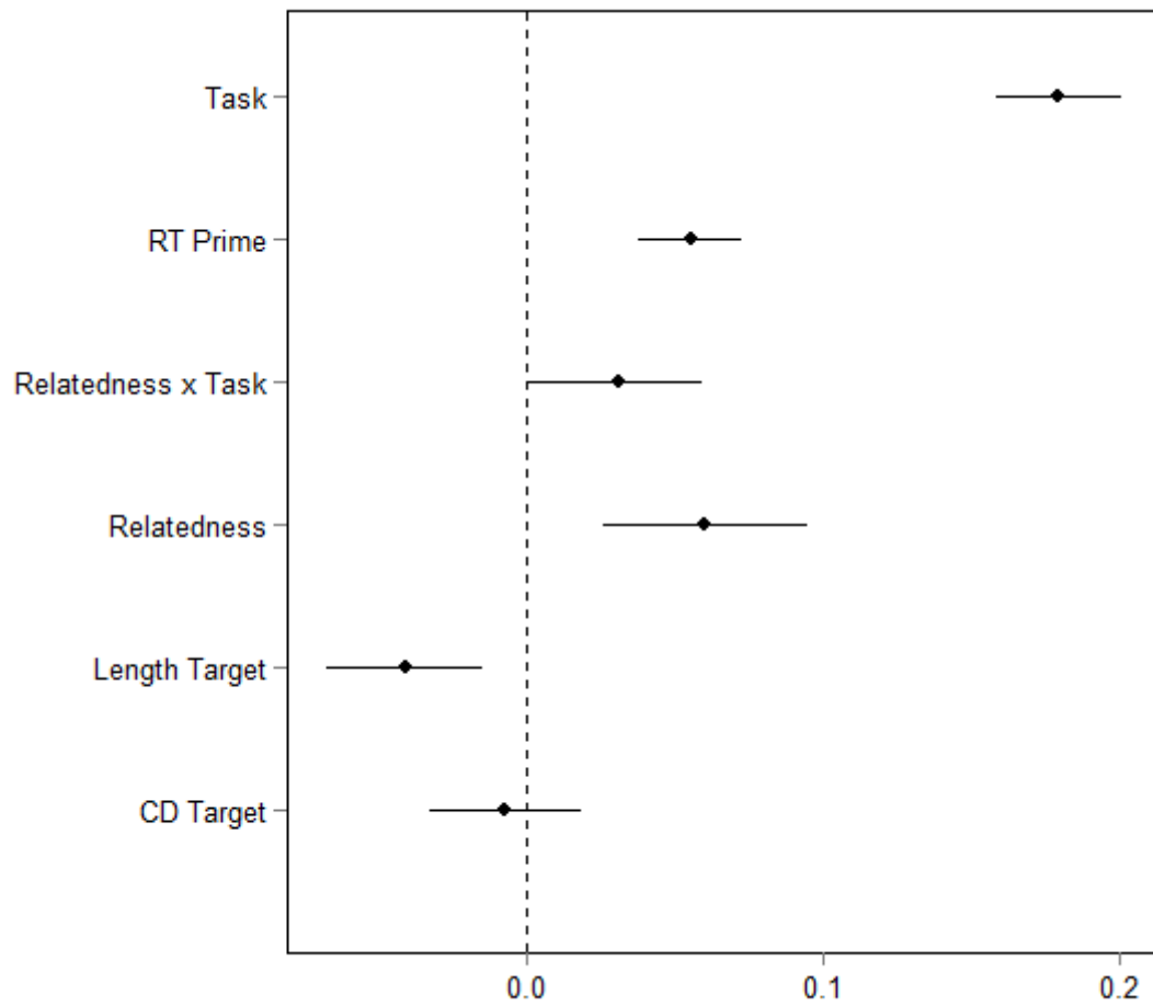
Figure 9. 95% highest posterior density intervals of the six regression weights. The diamonds represent the point estimates of the weights.
