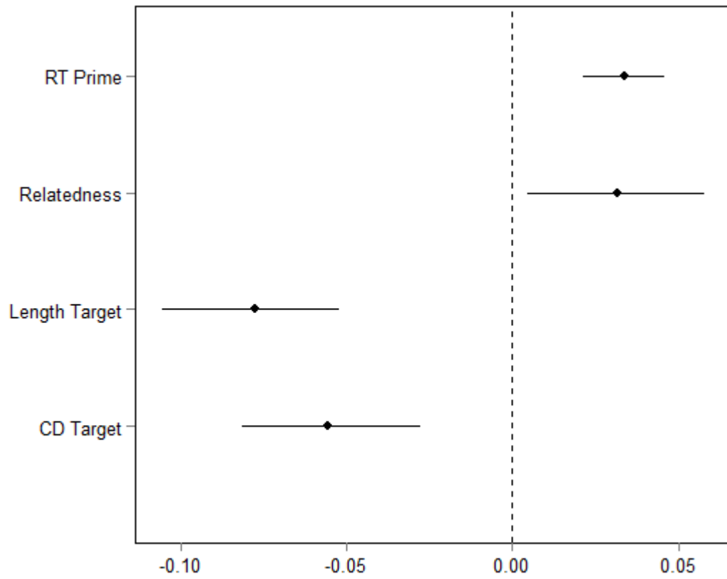
Figure 2. 95% highest posterior density intervals of the four regression weights. The diamonds represent the point estimates of the weights.
