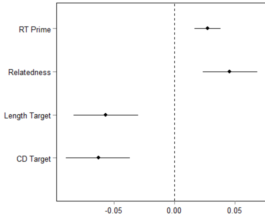
Figure 1. 95% highest posterior density intervals of the four regression weights. The diamonds represent the point estimates of the weights.
