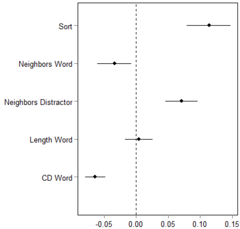
Figure 6. 95% highest posterior density intervals of the five regression weights for the data from Experiment 1. The diamonds represent the point estimates of the weights.
