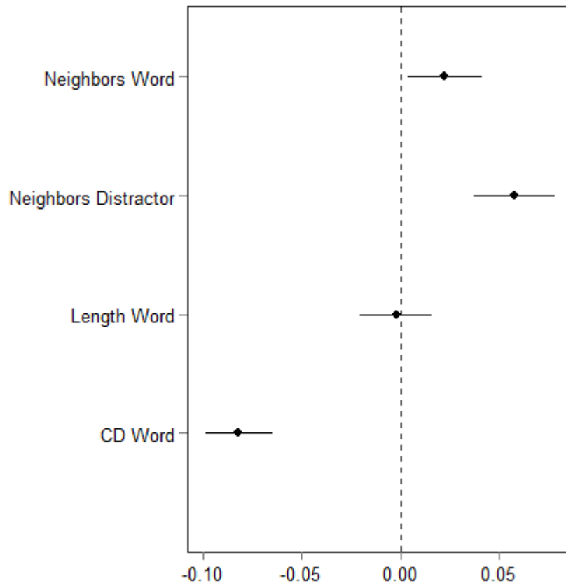
Figure 7. 95% highest posterior density intervals of the four regression weights for the data from Experiment 2. The diamonds represent the point estimates of the weights.
