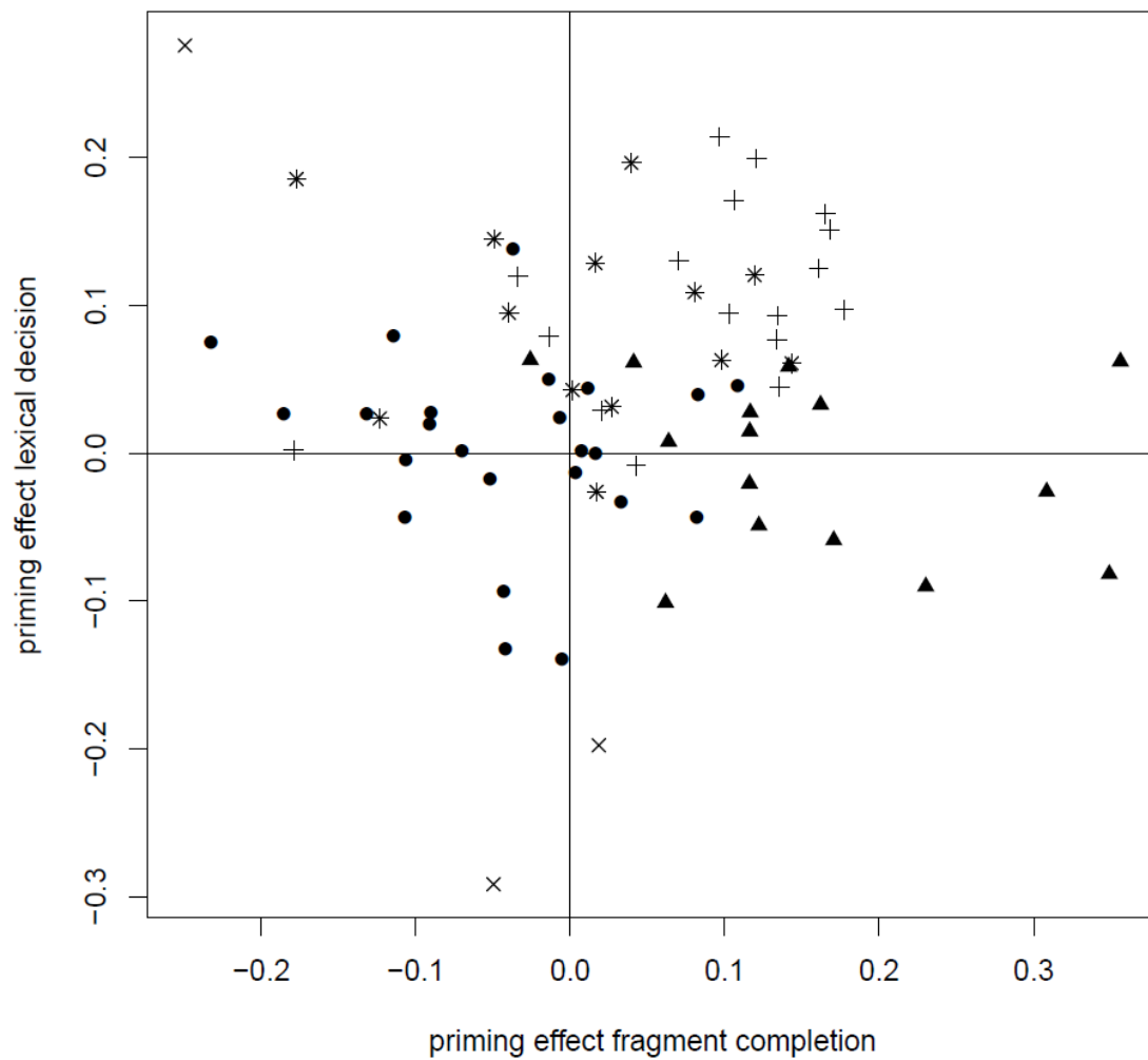
Figure 4. Priming effect per item in the speeded word fragment completion task plotted against the priming effect per item in the lexical decision task. Every symbol represents an item. The plus sign (+) represents items that require more time than average in both tasks, the dots are the items that take less time than average in both tasks, the star sign (*) are items completed faster than average in the speeded word fragment completion task, but recognized slower than average in the lexical decision task and vice versa for the triangles. The x sign are items that were not recognized as words by more than 10 participants.
