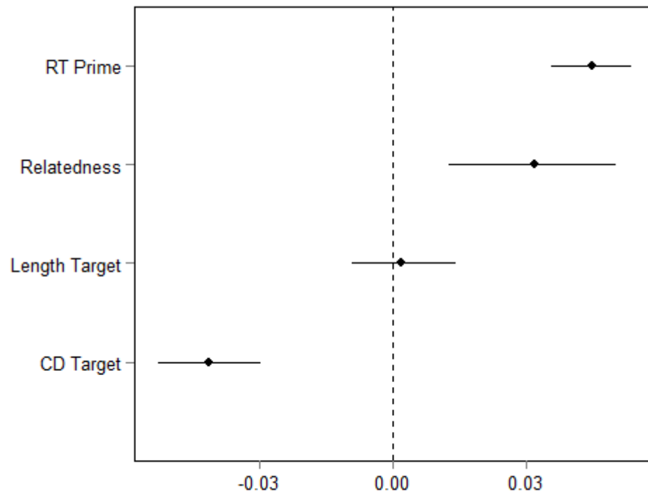
Figure 3. 95% highest posterior density intervals of the four regression weights. The diamonds represent the point estimates of the weights.
